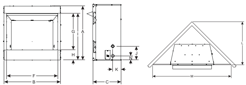
Flush Fireboxes
