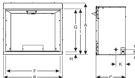
Select Fireboxes
