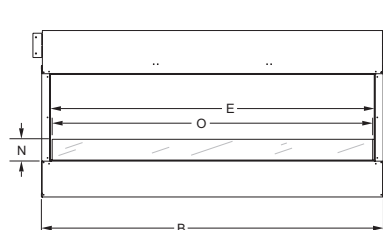
See-Through 60-inch Fireplace
