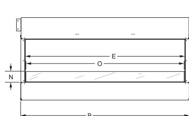
Single-Sided 60-inch Fireplace
