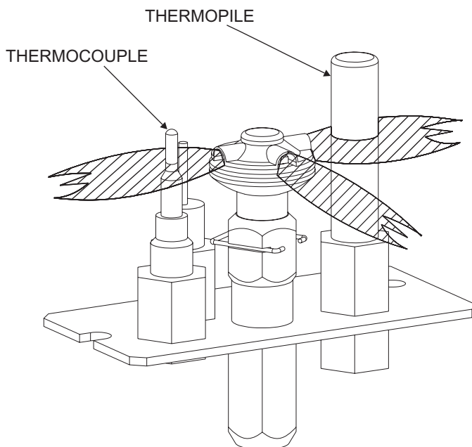
PILOT ASSEMBLY
