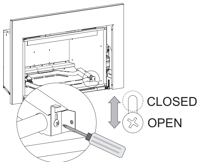
Front Air Shutter Adjustment
