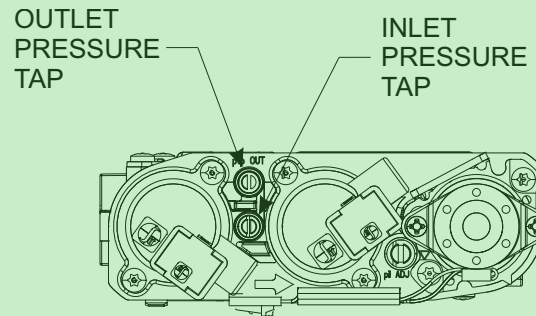
Figure 6 - IP Valve
