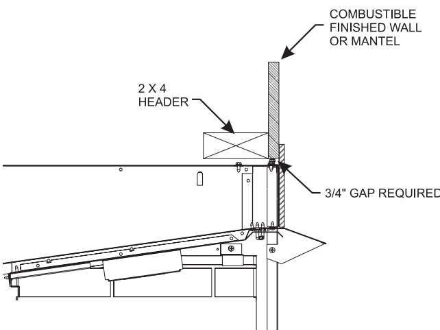
Figure 3 - Flush Models
