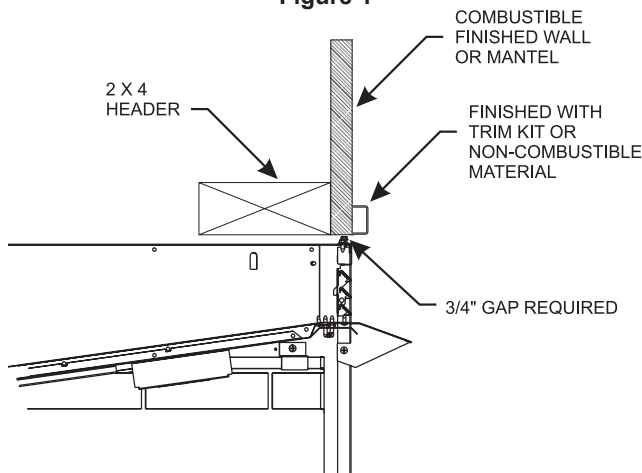
Figure 2 - Louvered Models
